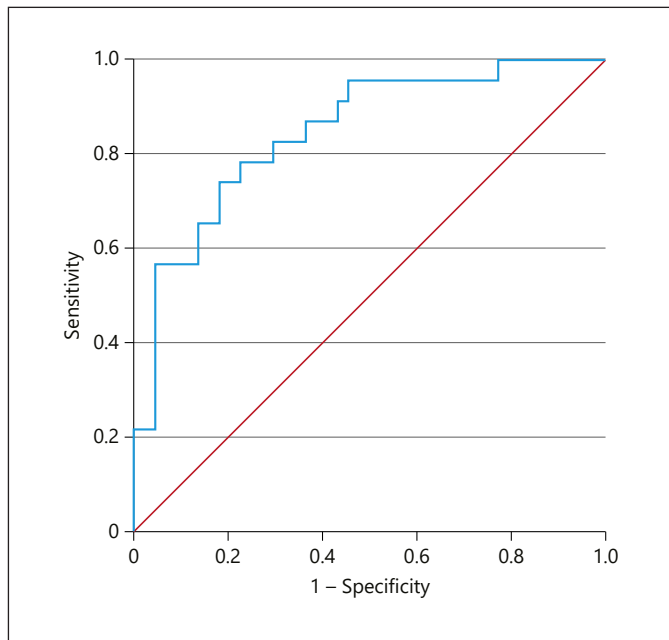
Fig. 2. ROC curve of beta-glucuronidase activity. AUC, area under the curve; CI, confidence intervals. AUC 0.846 (95% CI 0.748–0.943).
