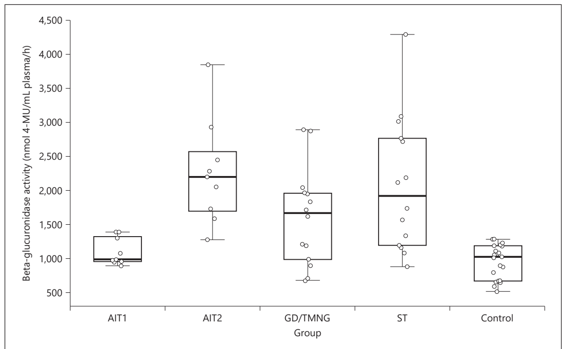
Fig. 1. Box plot of plasma beta-glucuronidase activity for each one of the study groups. Small circles: each individual's value. Rectangle: 25th–75th percentile. Horizontal line within the rectangle: median. Whiskers: minimum and maximum.
