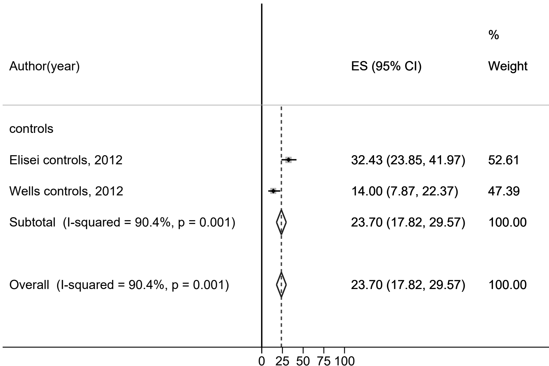
Supplement figure 5. Proportion of MTC control patients with Grade \geq 3 Adverse Events (G3AEs). G3AEs were reported in 23.7% [95%CI 17.8 – 29.5; Q=10.4 , X^2(d.f. 1) , p=0.001 , I^2=90.4\% ] of patients ( z=7.9 , p<0.001 )
